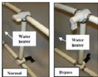
Two Valve Water Heater Bypass
